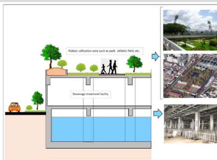
Figure 15.3.2 Conceptual Image of Sewerage Treatment Plant (half underground type)
