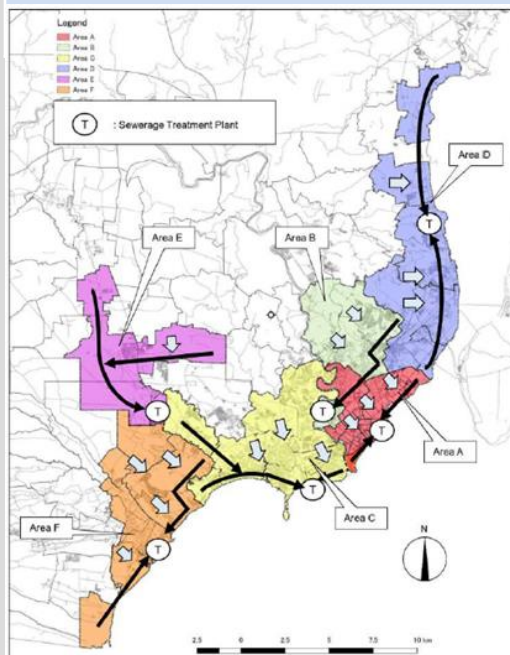
Figure 15.3.1 Sewerage Treatment Areas
